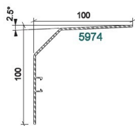
CORNIERE ALUMINIUM 100X100 W04
