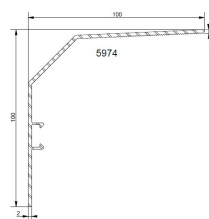
CORNIERE ALUMINIUM 100X100
